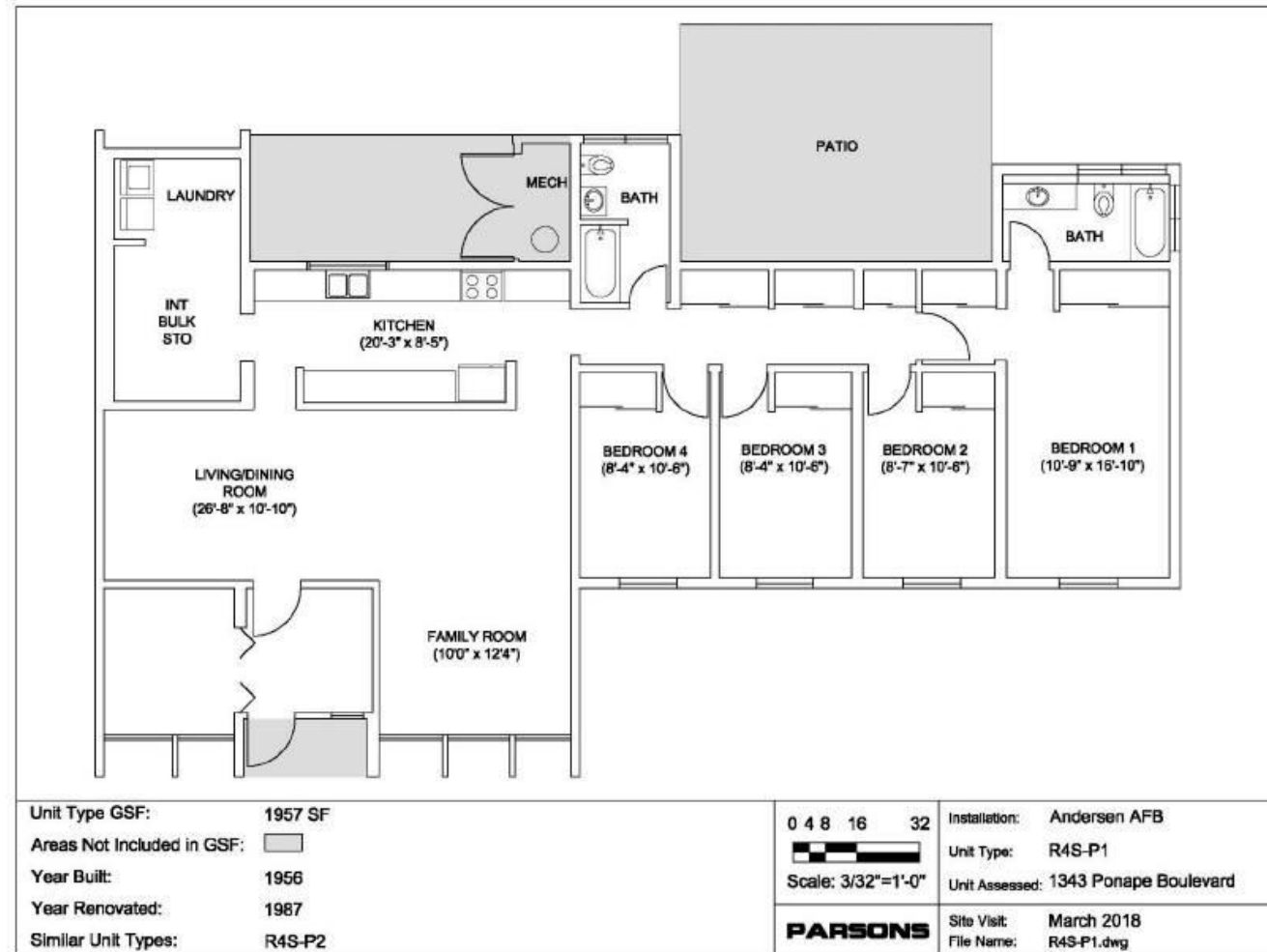
FIELD GRADE OFFICER 4 BEDROOM - R4S1/R4S2
