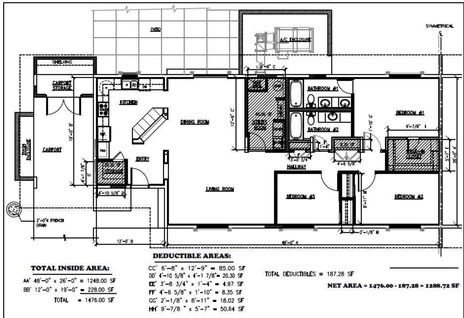
COMPANY GRADE 3 BEDROOM - CO3D10
