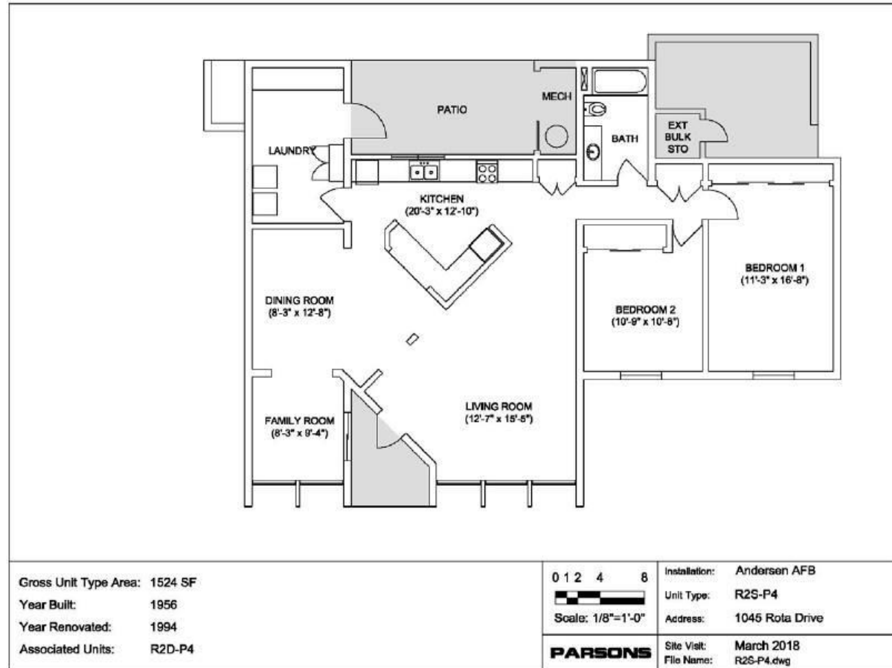
COMPANY GRADE OFFICER 2 BEDROOM - R2D4/R2S4
